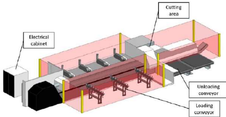
18. Figure Tube laser isometric view
