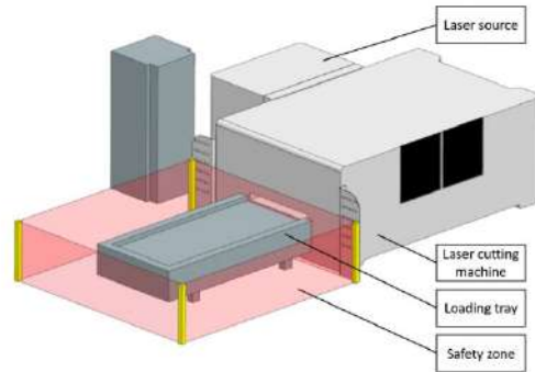
11. Figure Sheet laser cell isometric view
